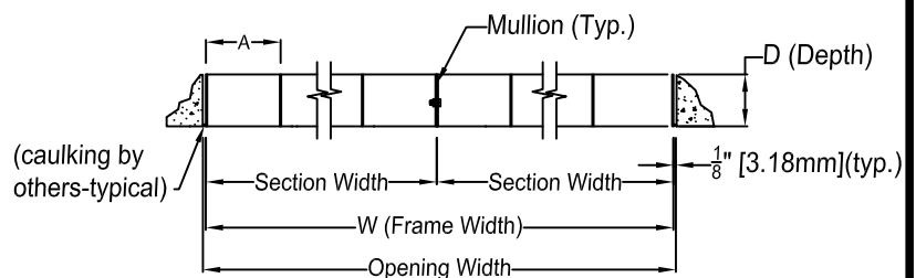
HORIZONTAL SECTION
